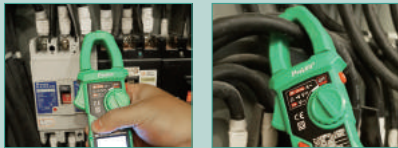
Non contact ACV detector ACA measurement
