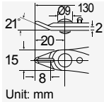
PM-107C Safety clip design prevents flying leads.
