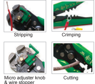
Micro adjuster knob & wire stopper
