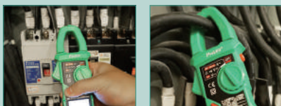
Non contact ACV detector ACA measurement
