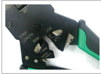
Stripping twisted pair round cable
