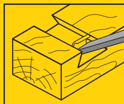
Dovetail joints
